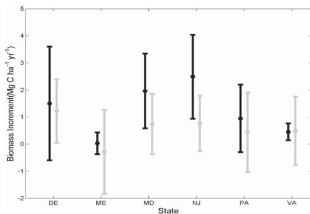
Figure 4. State-level biomass increment ( \text{Mg C ha}^{-1} \text{ yr}^{-1} ) estimated using data from the U.S. Forest Service FIA program (black) and TEM (gray) for Delaware (DE), Maine (ME), Maryland (MD), New Jersey (NJ), Pennsylvania (PA), and Virginia (VA). Error bars represent standard deviations of variation among plots for the inventory estimates and among cohorts for the TEM estimates.
