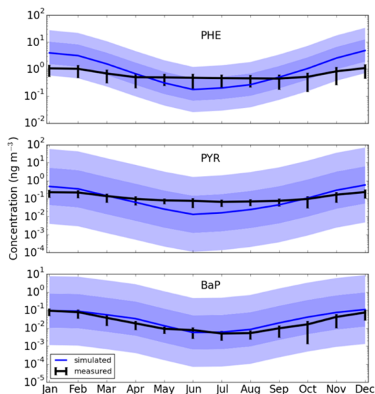
Figure 1. Measured and simulated total (gas and particulate) concentrations at nonurban sites for PHE (top), PYR (middle), and BaP (bottom). The black lines are means across the measurements at all nonurban sites, and their error bars show the standard deviation of the mean for each month. The blue lines are the simulated means across the same sites, with the shaded regions marking the \sigma and 2\sigma intervals of the parametric uncertainty distributions for each month.
