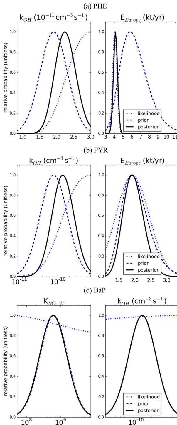
Figure 2. Constraint of parameter uncertainty distributions by measurement data. (a) PHE, (b) PYR, (c) BaP distributions for the two most important parameters each. Prior distributions (dashed lines), observation-based likelihoods (dot-dashed lines), and posterior distributions (solid lines) shown.
