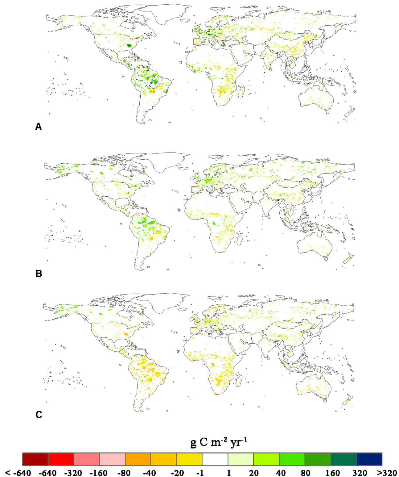
Fig. 4 Carbon sequestration rates by land ecosystems for current conditions (2005–2010) and under two future scenarios at the end of the twenty-first century (2095–2100): A current conditions; B the FP scenario; and C the NP scenario. In the FP scenario, the extent of protected areas is constant over the twenty-first century, while in the NP scenario, the extent of protected areas is reduced in response to land-use pressures from a growing and wealthier world population
