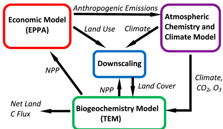
Fig. 1 The dynamically linked modeling system. It consists of an economic model (EPPA), a terrestrial biogeochemistry model (TEM) using climate output from an atmospheric chemistry and climate model (Reilly et al. 2012). The creation of plant biomass, known as net primary production (NPP) is calculated within TEM as the difference between GPP and R_A (see text). Within the modeling system, the combination of TEM and the atmospheric chemistry and climate models are referred to as the MIT Earth Systems Model (MESM)
