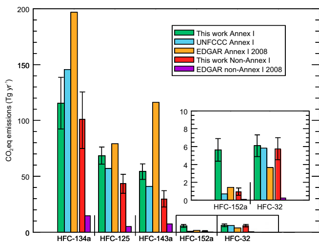
Fig. 3. Mean emissions during 2010–2012 of each HFC inferred for all Annex I countries (green) and non-Annex I countries (red). Also shown are the Annex I UNFCCC inventory (blue), EDGAR Annex I (orange), and EDGAR non-Annex I estimates (violet). EDGAR values are for 2008, the last year of available data. Uncertainty bars reflect the fifth to 95th percentile of the inferred emission estimates.
