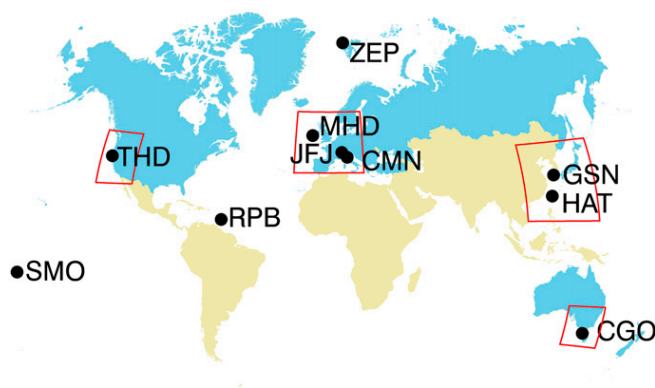
Fig. 1. Location of AGAGE and NIES stations, showing, from north to south: ZEP, Ny Ålesund, Norway; MHD, Mace Head, Ireland; JFJ, Jungfrauoch, Switzerland; CMN, Mt. Cimone, Italy; THD, Trinidad Head, United States; GSN, Gosan, South Korea; HAT, Hateruma, Japan; RPB, Ragged Point, Barbados; SMO, Cape Matatula, American Samoa; and CGO, Cape Grim, Australia. Red boxes indicate local regions where the NAME model was used with increased resolution compared with the global MOZART model, which was run for the remainder of the globe. Annex I countries are shaded blue, and non-Annex I are in pale yellow.
