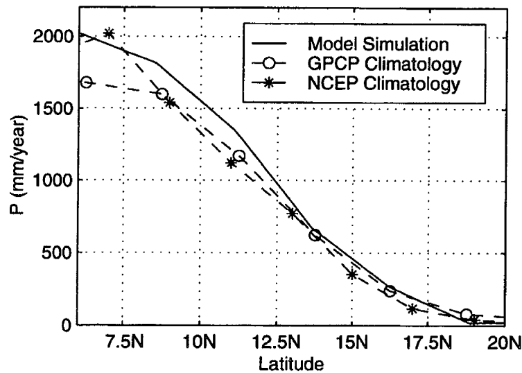
Figure 3-8: Comparison of the annual rainfall (in mm/year ) between the model simulation (solid line), the GPCP climatology (— o —), and the NCEP climatology (— * —).
