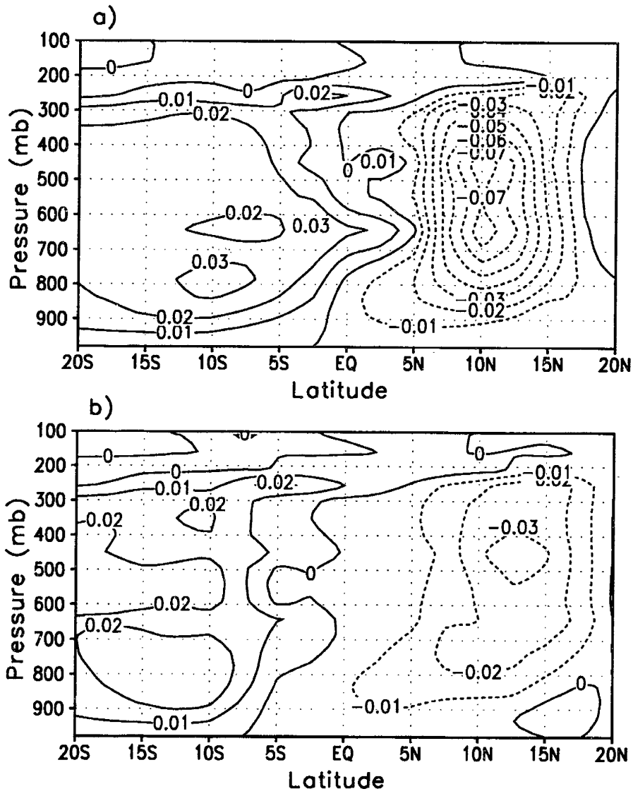
Figure 4-8: Vertical velocity during August, in \text{Pa}/\text{sec} . a) for the variable case; b) for the uniform case.
