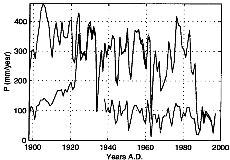
Figure 6-10: Time series of the annual rainfall at the grid point near 16°N, in the Wet2 experiment (green) and the Dry2 experiments starting from 1898 (blue) and 1938 (red).
