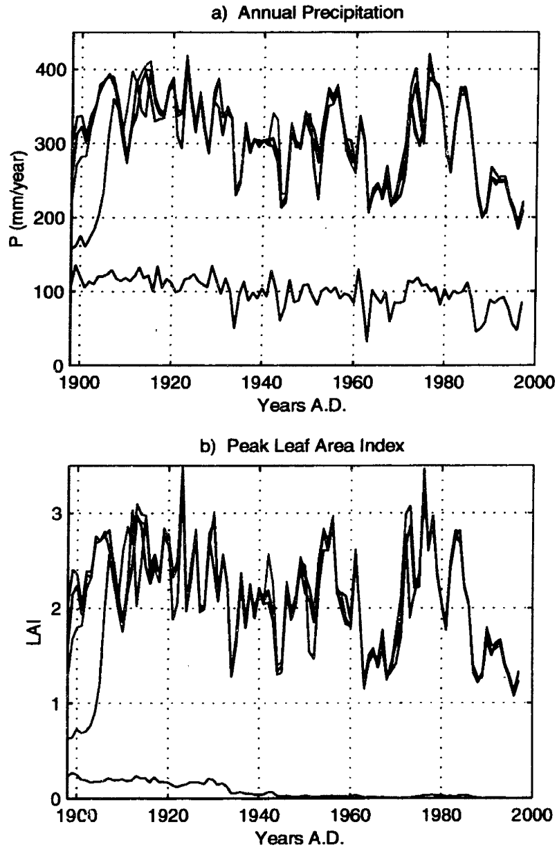
Figure 6-7: Time series of (a) the annual rainfall and (b) the growing-season LAI at the grid point near 16^{\circ}\text{N} , in the control simulation Dyn-Control (black) and sensitivity experiments Dyn-Pert1 (green), Dyn-Pert2 (blue), Dyn-Pert3 (magenta), and Dyn-Pert4 (red).
