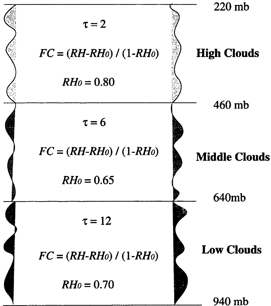
Figure 2-1: A summary of the cloud parameterization scheme. Here \tau is the cloud optical depth, and the definition for RH and RH_0 is the same as in Eq. (2.11). FC is first calculated at each pressure level based on the relative humidity at the corresponding level. The average of FC within the vertical extent of each cloud type is then used as the fractional cover for that type of clouds.
