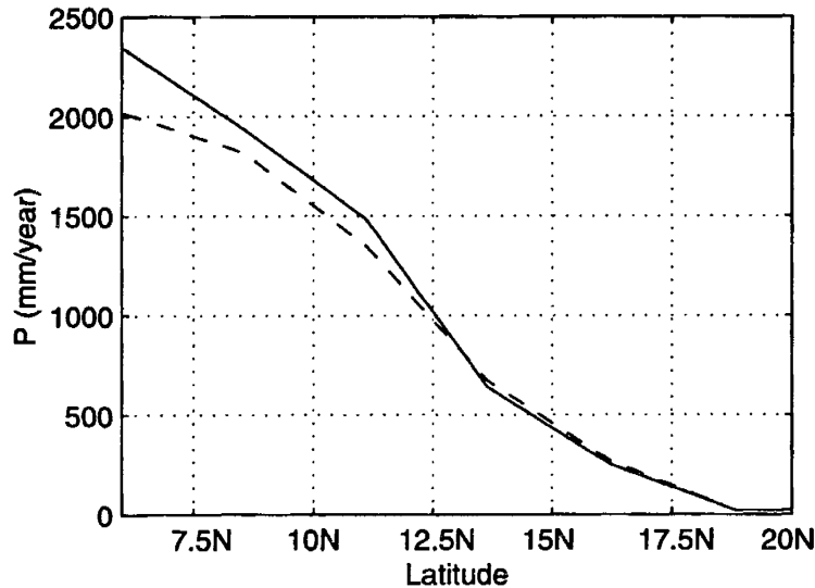
Figure 3-23: The meridional distribution of the annual rainfall (in mm/year ), at the attained biosphere-atmosphere equilibrium (solid line). As a comparison, the dashed line plots the rainfall distribution modeled with fixed, “close-to-current” vegetation.
