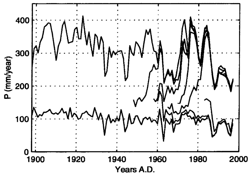
Figure 6-9: Time series of the annual rainfall at the grid point near 16°N. Green and red lines stand for the experiments that begin from different years with the initial condition at the model’s medium equilibrium “B”; black lines plot the wet regime ( Dyn-Control ) and the dry regime ( Dyn-Pert4 ) for references.
