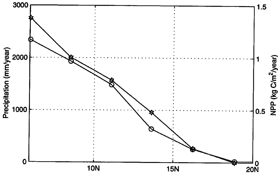
Figure 5-14: Precipitation (solid line with open circles) and NPP (solid line with hexagrams) at the control equilibrium state. This equilibrium is derived by starting the model with a vegetation distribution close to today's condition.
