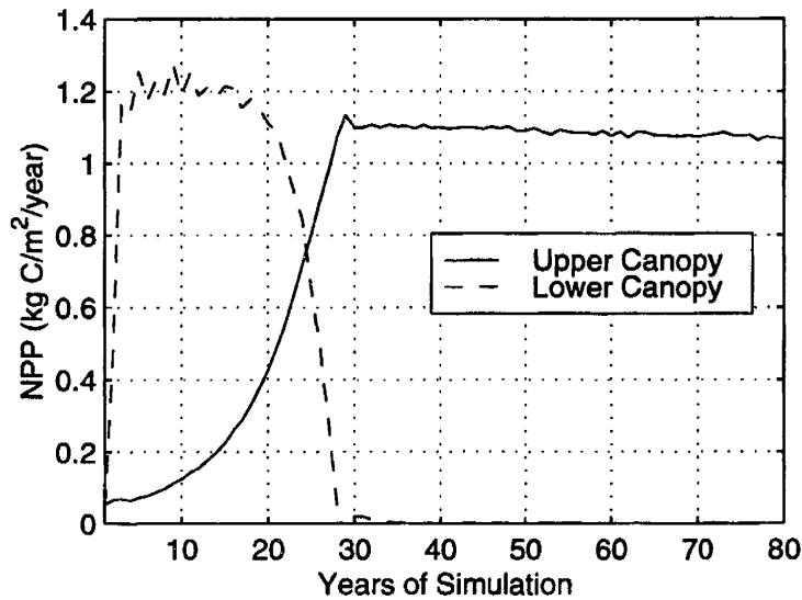
Figure 3-4: The net primary productivity (in \text{kgC}/\text{m}^2/\text{year} ) of the upper and lower canopy at 7^{\circ}N .
