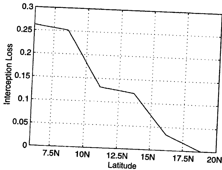
Figure 3-19: Interception loss as a fraction of the overall evapotranspiration.
