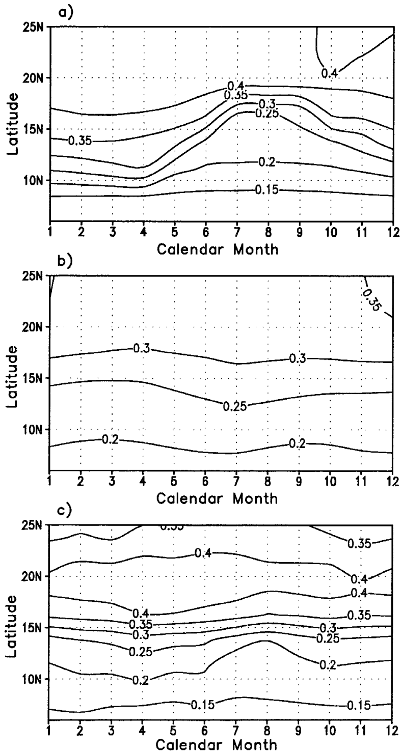
Figure 3-17: Seasonal cycle of the land surface albedo: a) model simulation; b) NCEP re-analysis data; c) ISCCP data.
