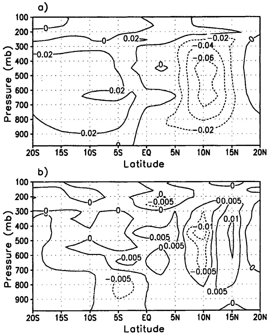
Figure 5-20: Vertical velocity ( \text{Pa/s} ) in August. a) Equilibrium "A"; b) The difference between equilibria "C" and "A": "C" - "A".
