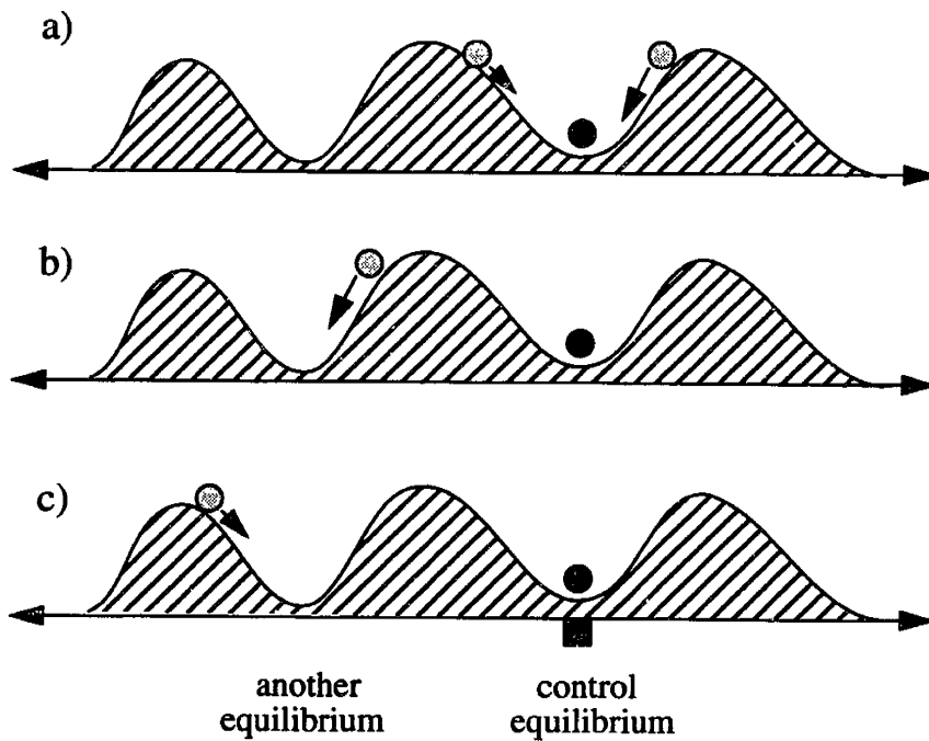
Figure 5-1: The movement of a ball on a simple landscape, as an analogy of the climate system with multiple equilibria. The three cases represent the system's responses to different perturbations: a) small perturbations: a negative feedback leads to a full recovery; b) larger perturbations: a positive feedback leads to a new equilibrium; c) perturbations even larger: a negative feedback leads to a new equilibrium.
