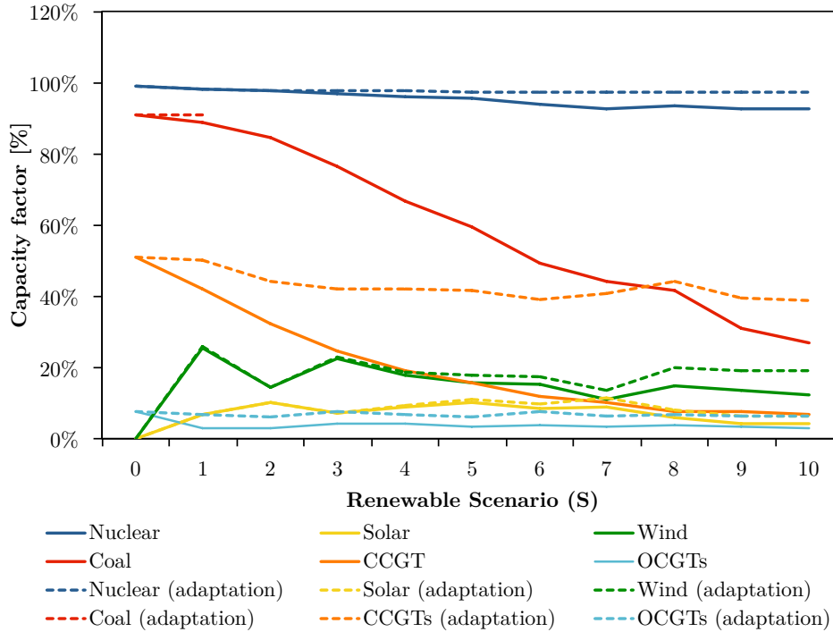
Figure 3-3: Capacity factor by technology under adaptation (dashed line) and non-adaptation (solid line).
