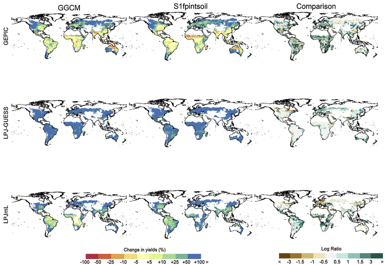
Fig. 11. Changes in rice yields from 2000 s to 2090 s estimated by the statistical emulators (S1fpintsoil specification) and GCMs and comparison (log ratio). Note: See note of Fig. 10.
